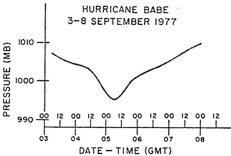
Figure 3. Lowest pressure vs time, 1977 Atlantic tropical cyclones
